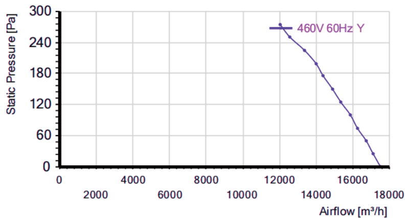
Characteristic curve
