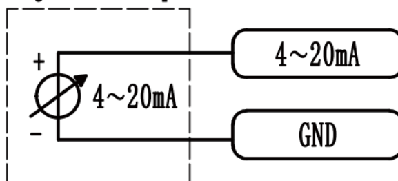
Adjustable speed via current
