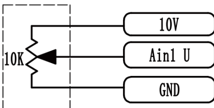
Adjustable speed via potentiometer
