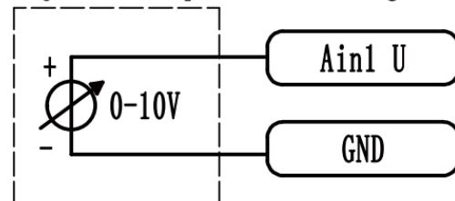
Adjustable speed via voltage/PWM
