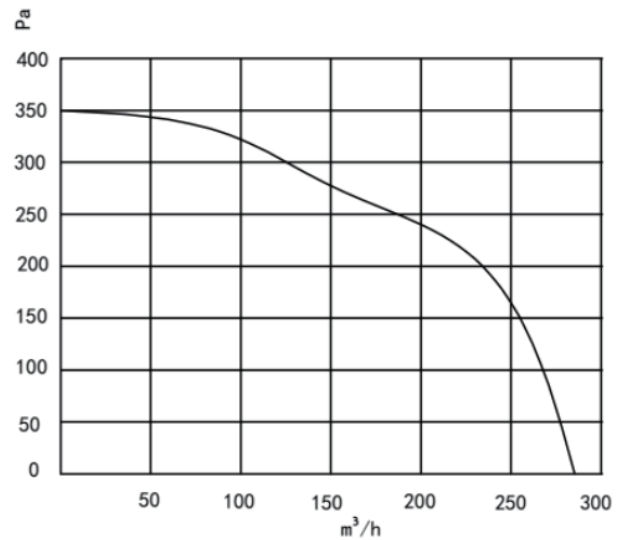
Air volume curve
