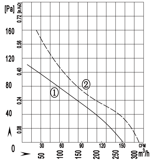
Air volume curve
