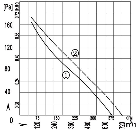
Air volume curve
