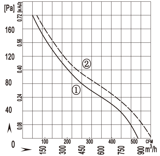
Air volume curve
